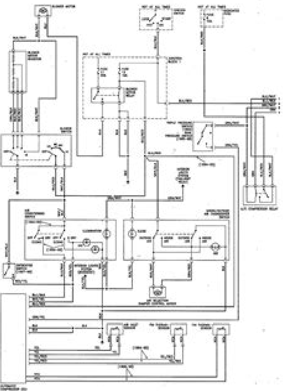
Heating and air conditioning system (manual) - 1990 and earlier models (1 of 2)
