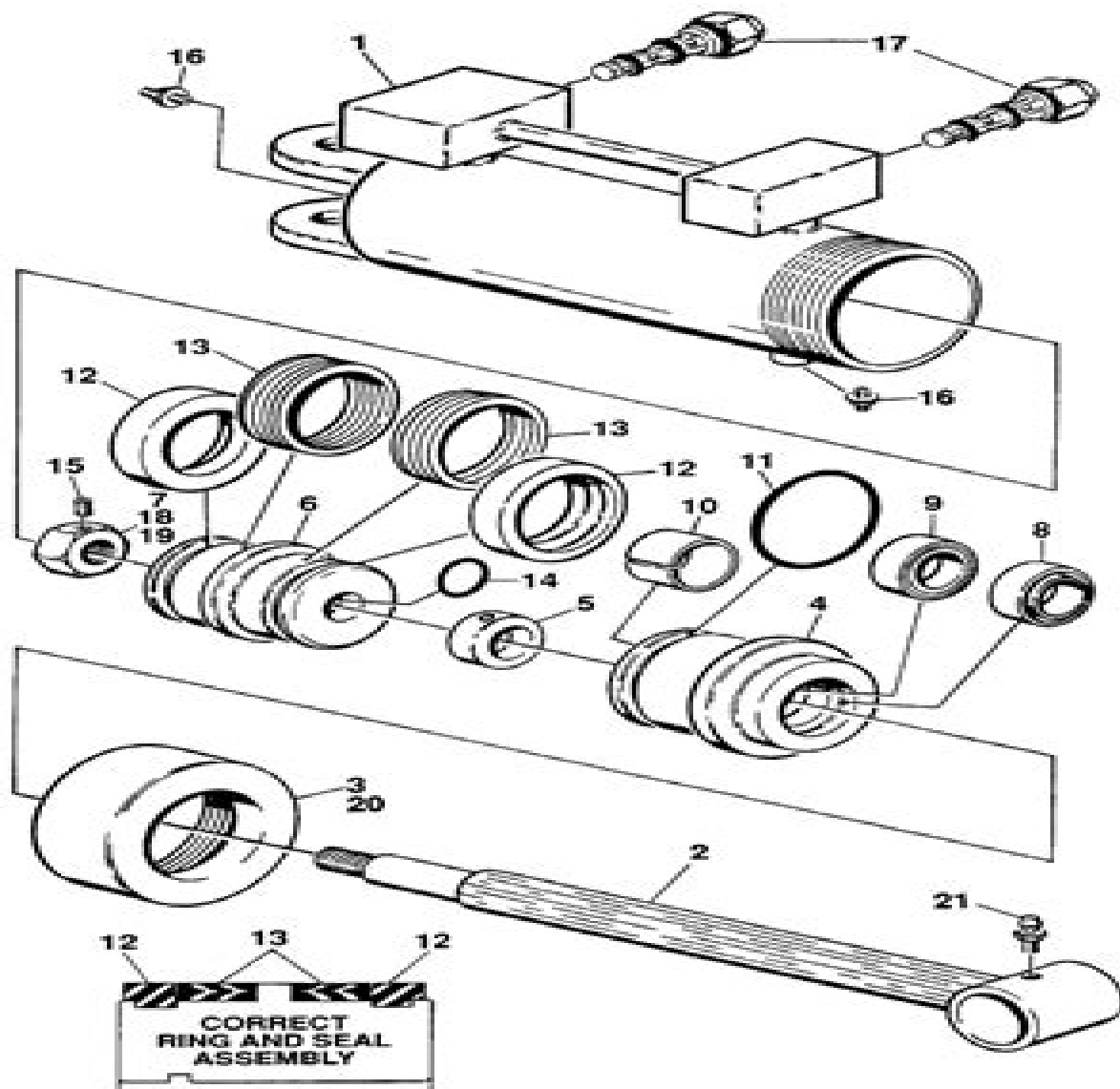
FIGURE 5-2. AXLE LOCKOUT CYLINDER ASSEMBLY
