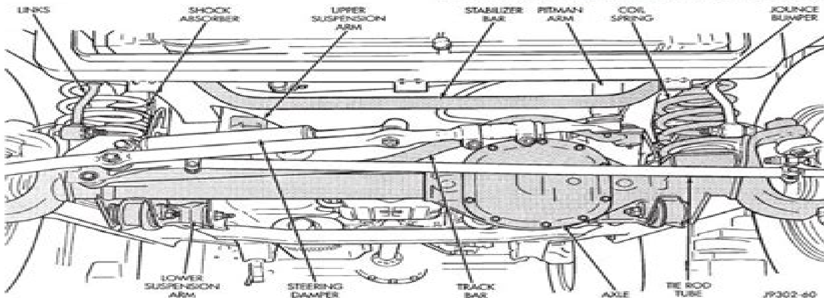
Fig. 1 Front Suspension
