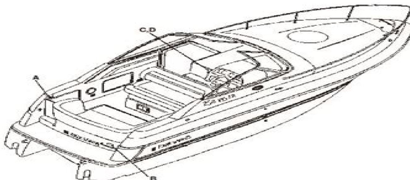
Figure 1: Vista Models
