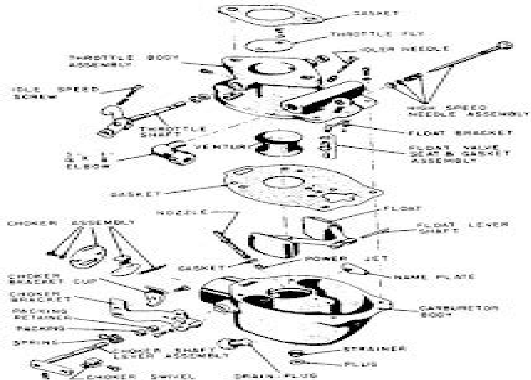
Fig. 5-12 Marvel-Schebler—Exploded
