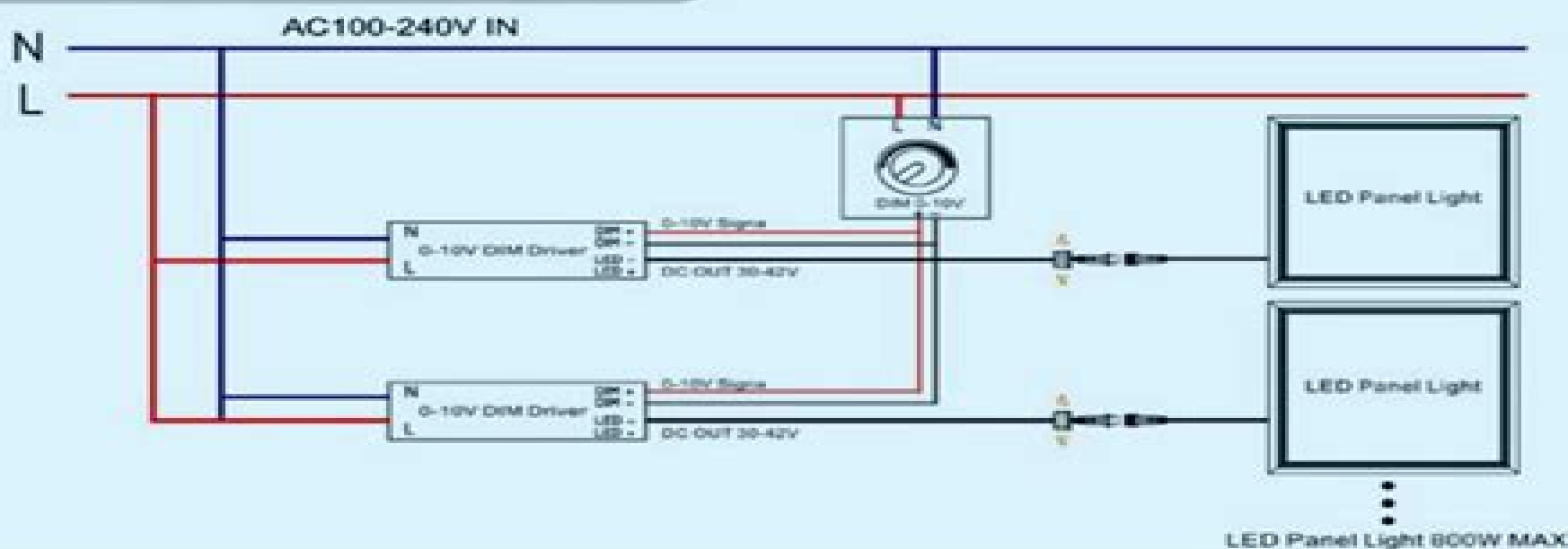
0-10Vdimming control wiring diagram 2
