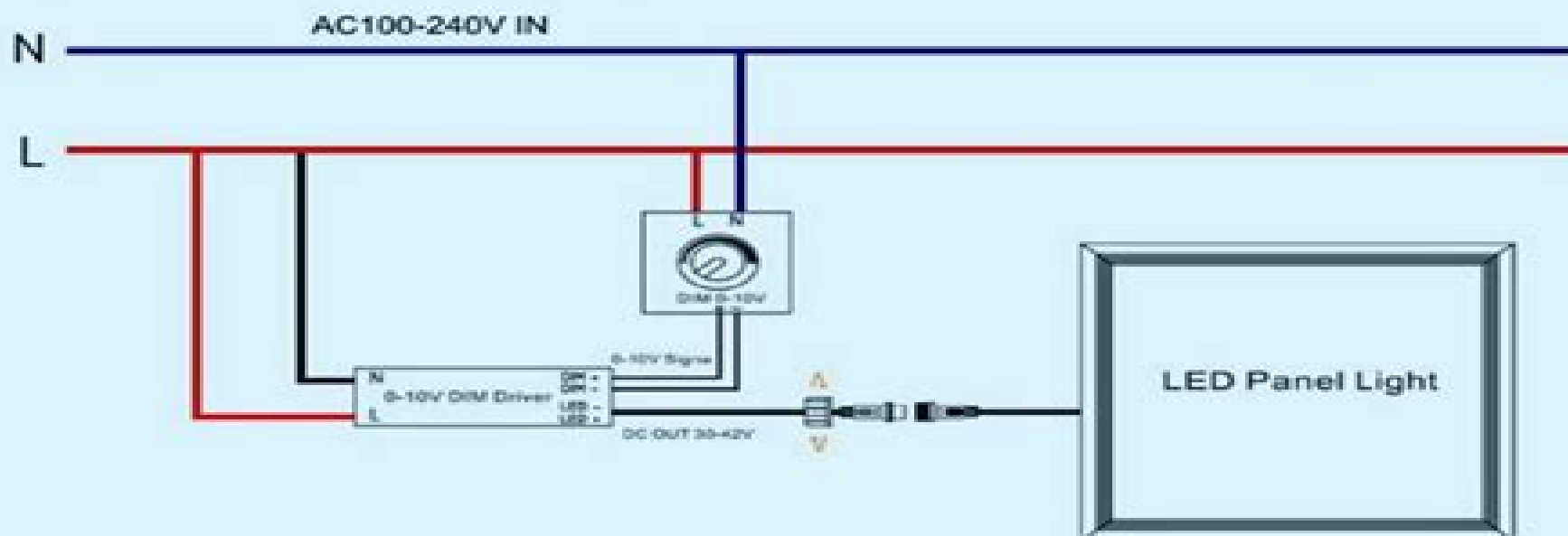
0-10Vdimming control wiring diagram 1
