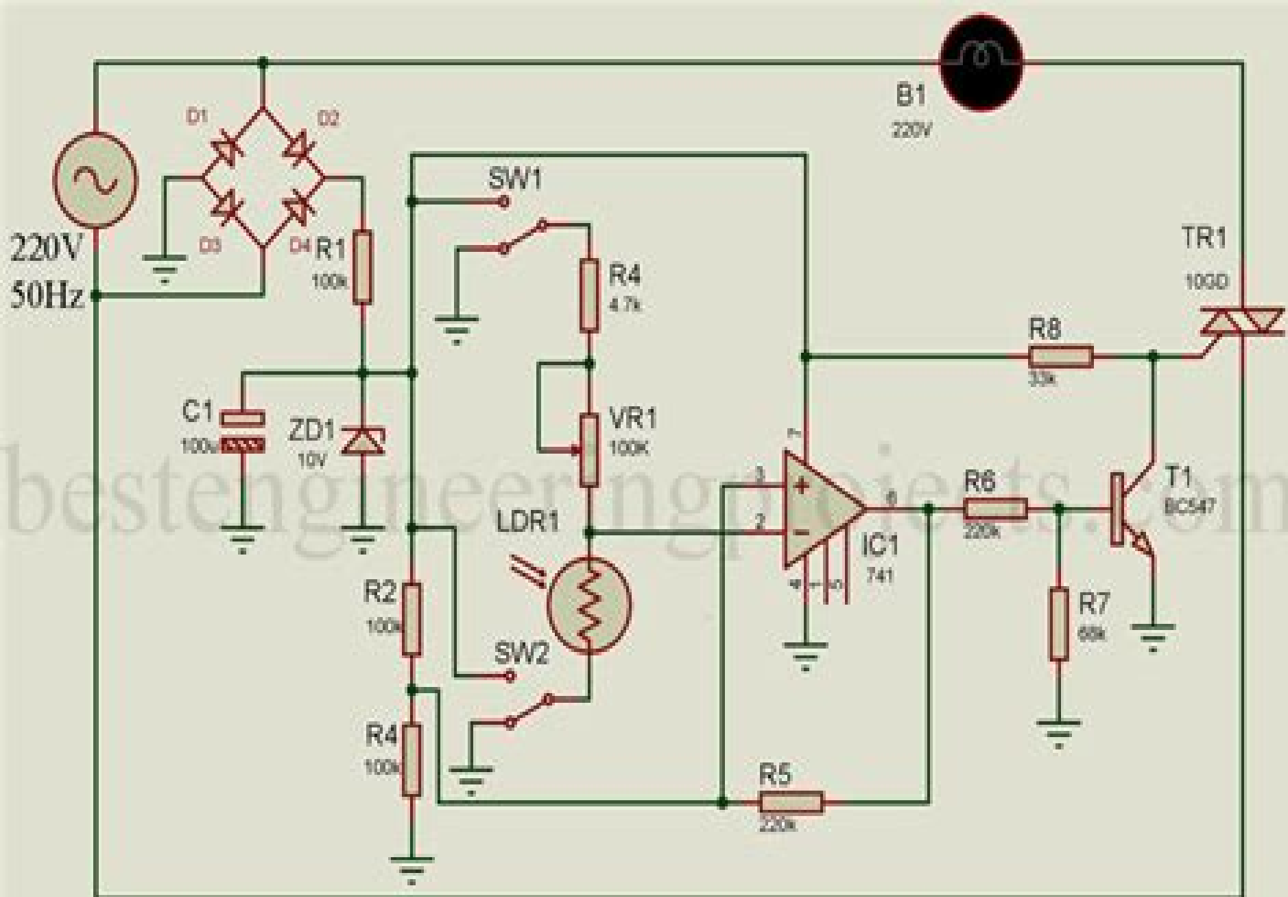
Figure 1: Light Sensitive Switch Circuit using Op-amp 741
