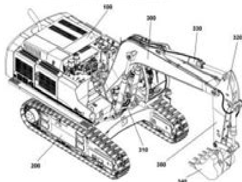
Fig. 1-1 Machine with backhoe attachment
