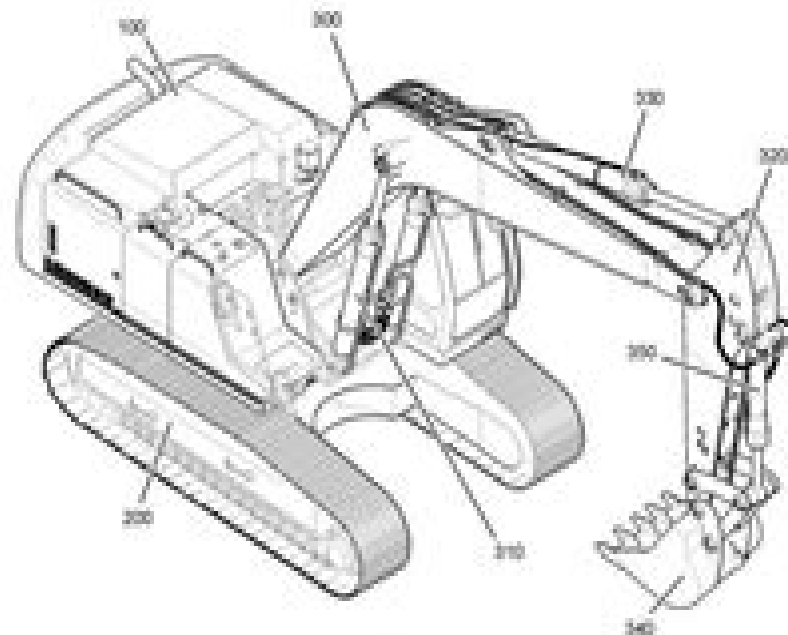
Fig. 1-1 Machine with backhoe attachment
