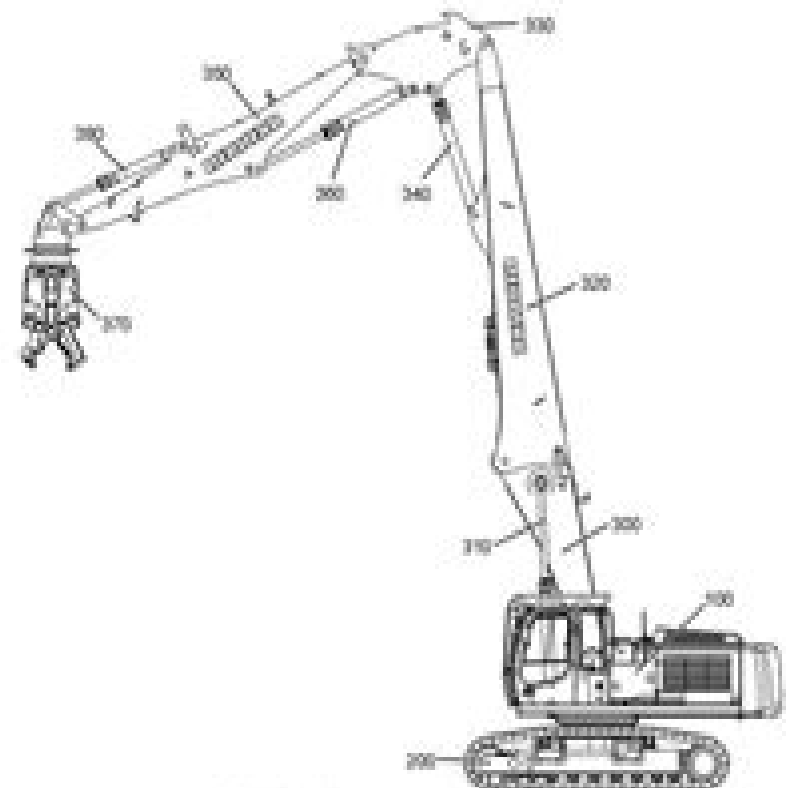
Fig. 1-2 Machine with demolition attachment
