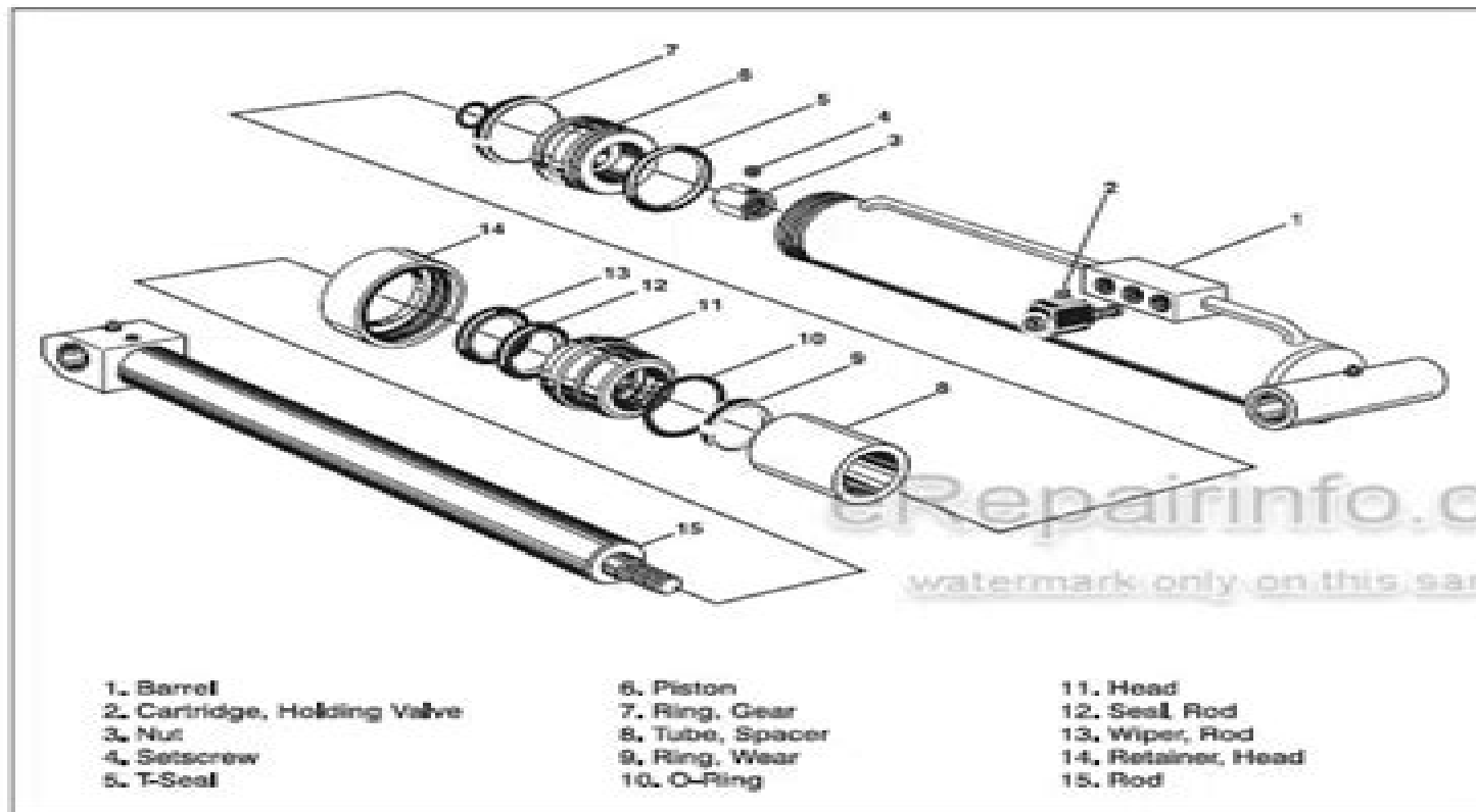
Figure 2-14. Lift Cylinder
