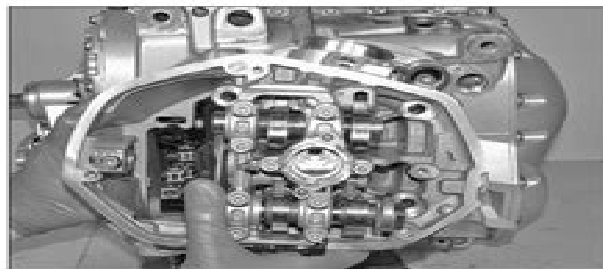
10.11 Remove the cylinder head
