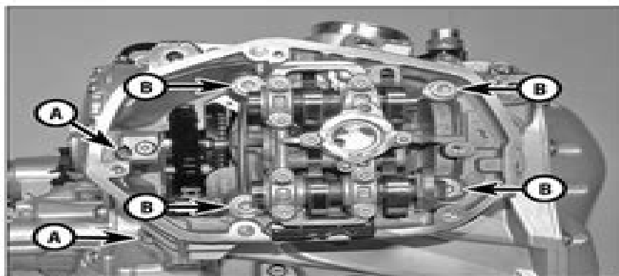
10.9 6mm bolts (A), 10mm bolts (B)
