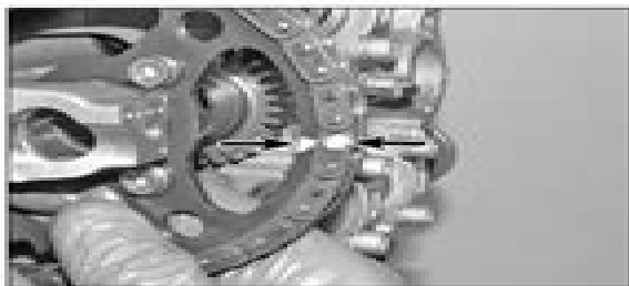
9.7a Make sure the mark made on the chain aligns with that on the sprocket
