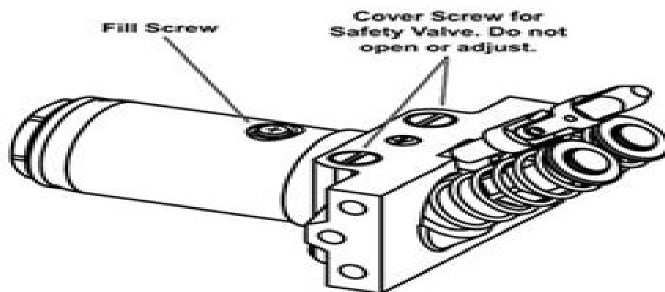
Figure B: Hydraulic Unit
