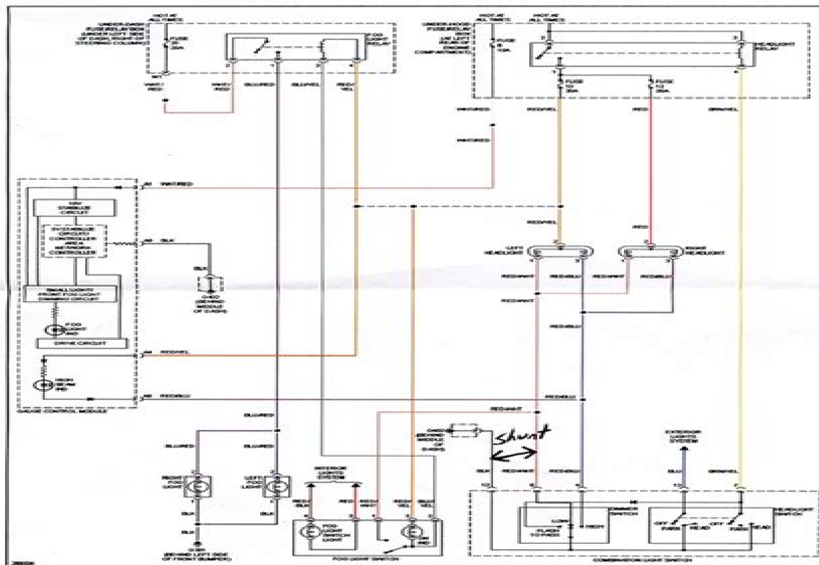
2007 Honda Fit-Fig. 27: Headlights Circuit, Fit W/O DRL
