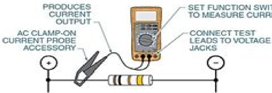
DMM WITH AC CLAMP-ON CURRENT PROBE ACCESSORY
