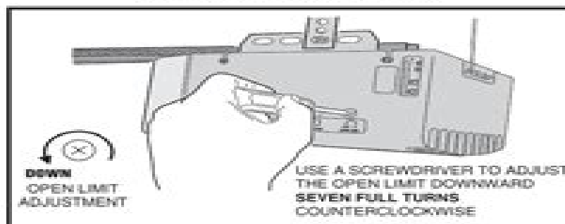
Adjusting the Open Limit on an LDO Operator
