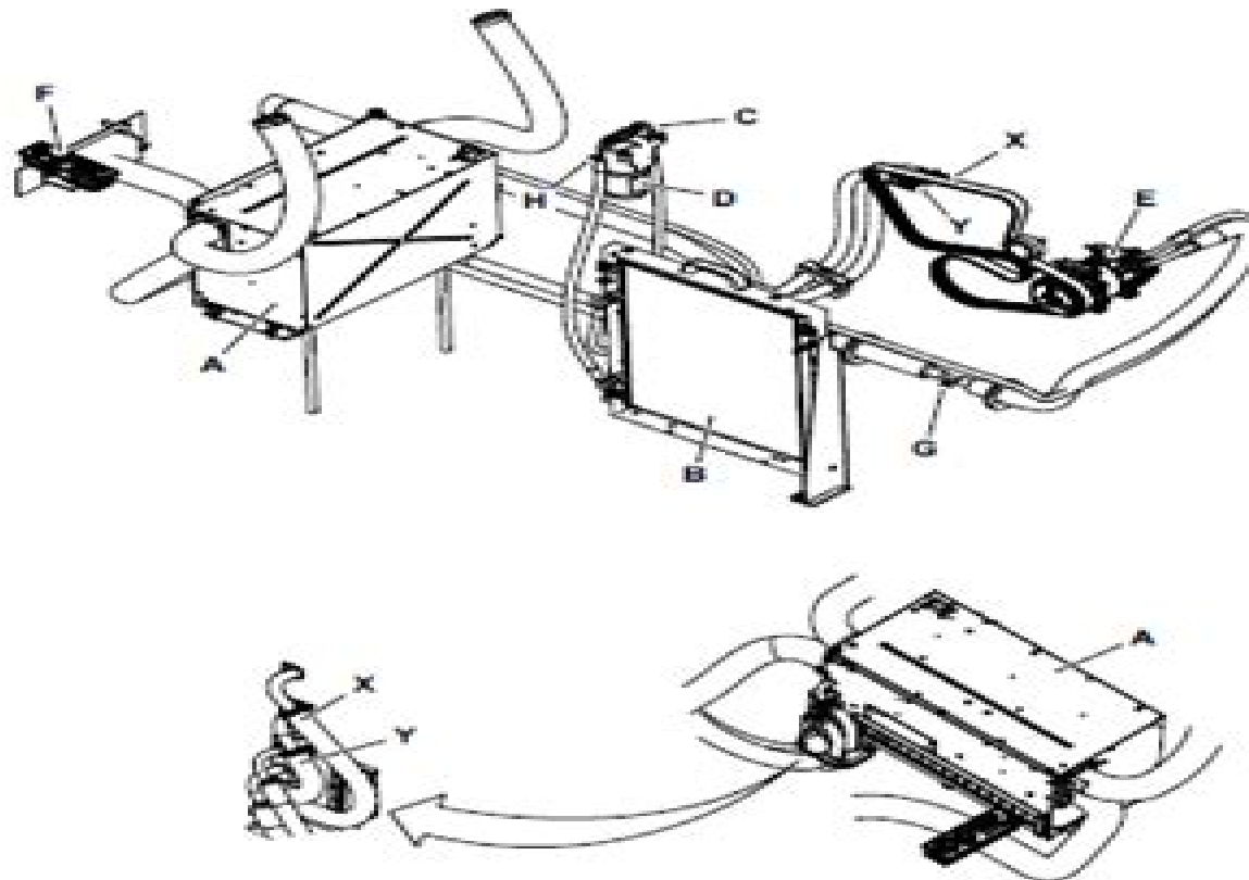
Fig. 1. System components: JS-116, JS-120, JS-146
