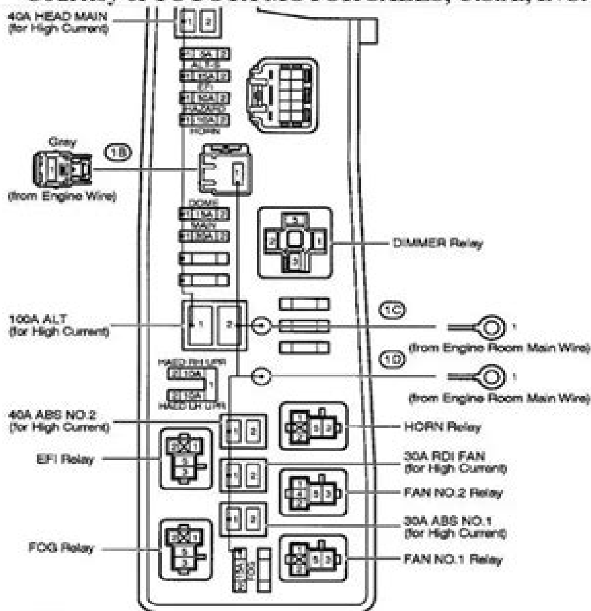
Fig. 3: Identifying Engine Compartment Junction & Relay Block Components Courtesy of TOYOTA MOTOR SALES, U.S.A., INC.
