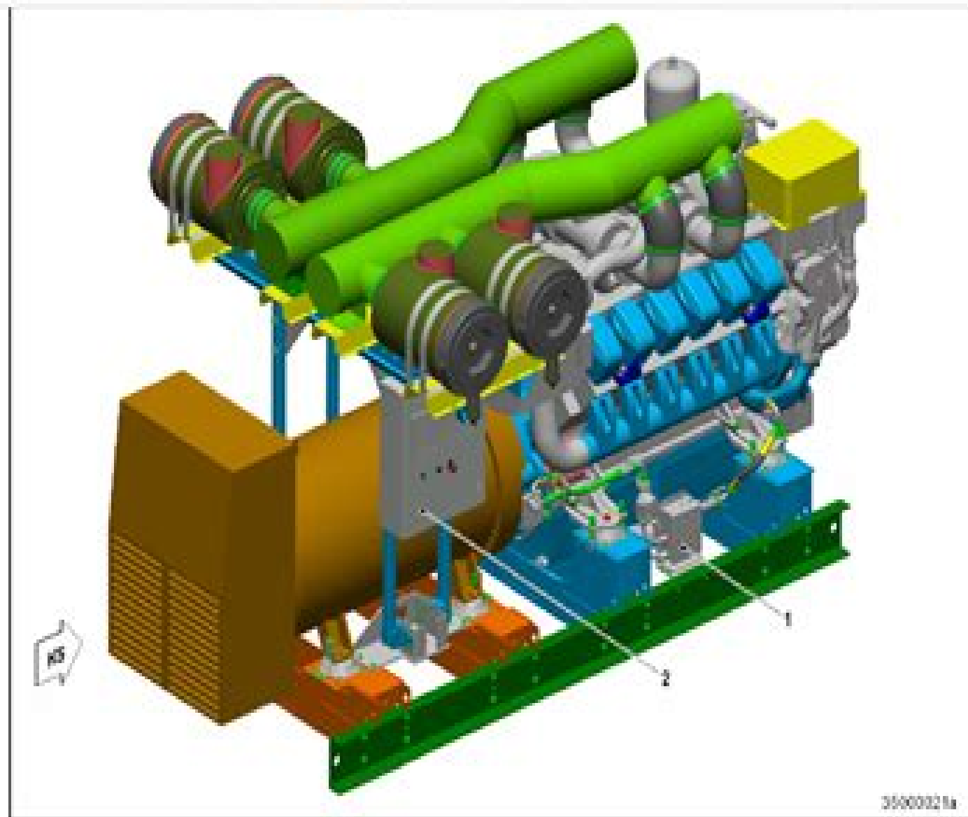
Figure 6: Engine-generator set with S4000 Gx3 engine – view on driving end
