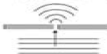
DIFFRACTION
