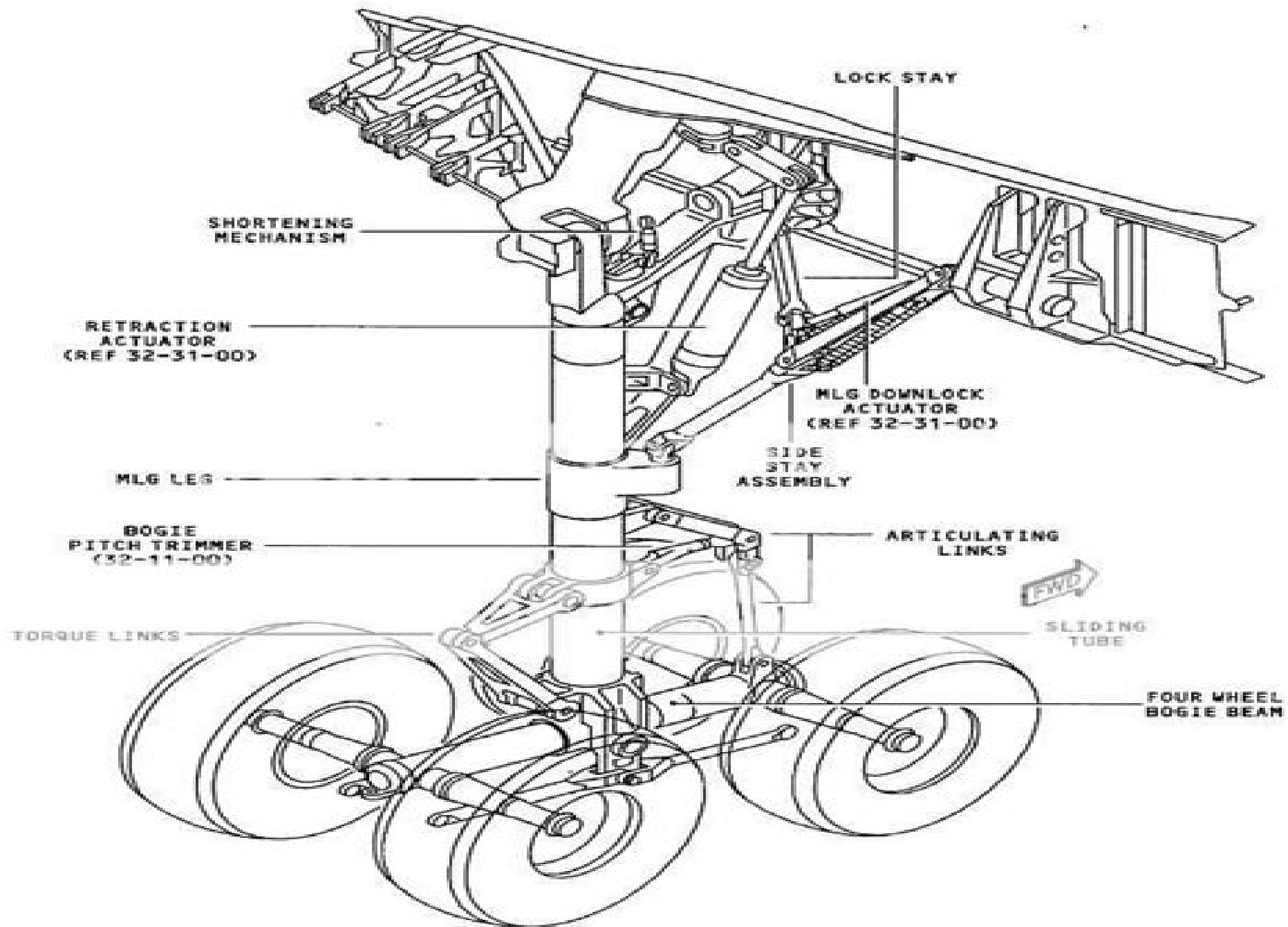
Main Landing Gear
