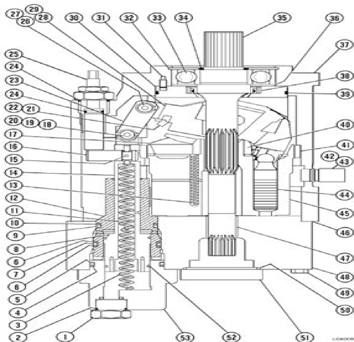
FIGURE 4-11. STEERING PUMP
