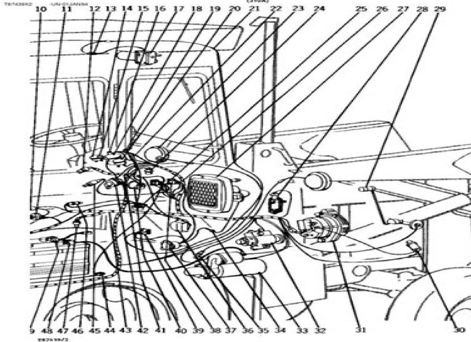
FIG. 3-ELECTRICAL SYSTEM - PART 2 (CONT.)
