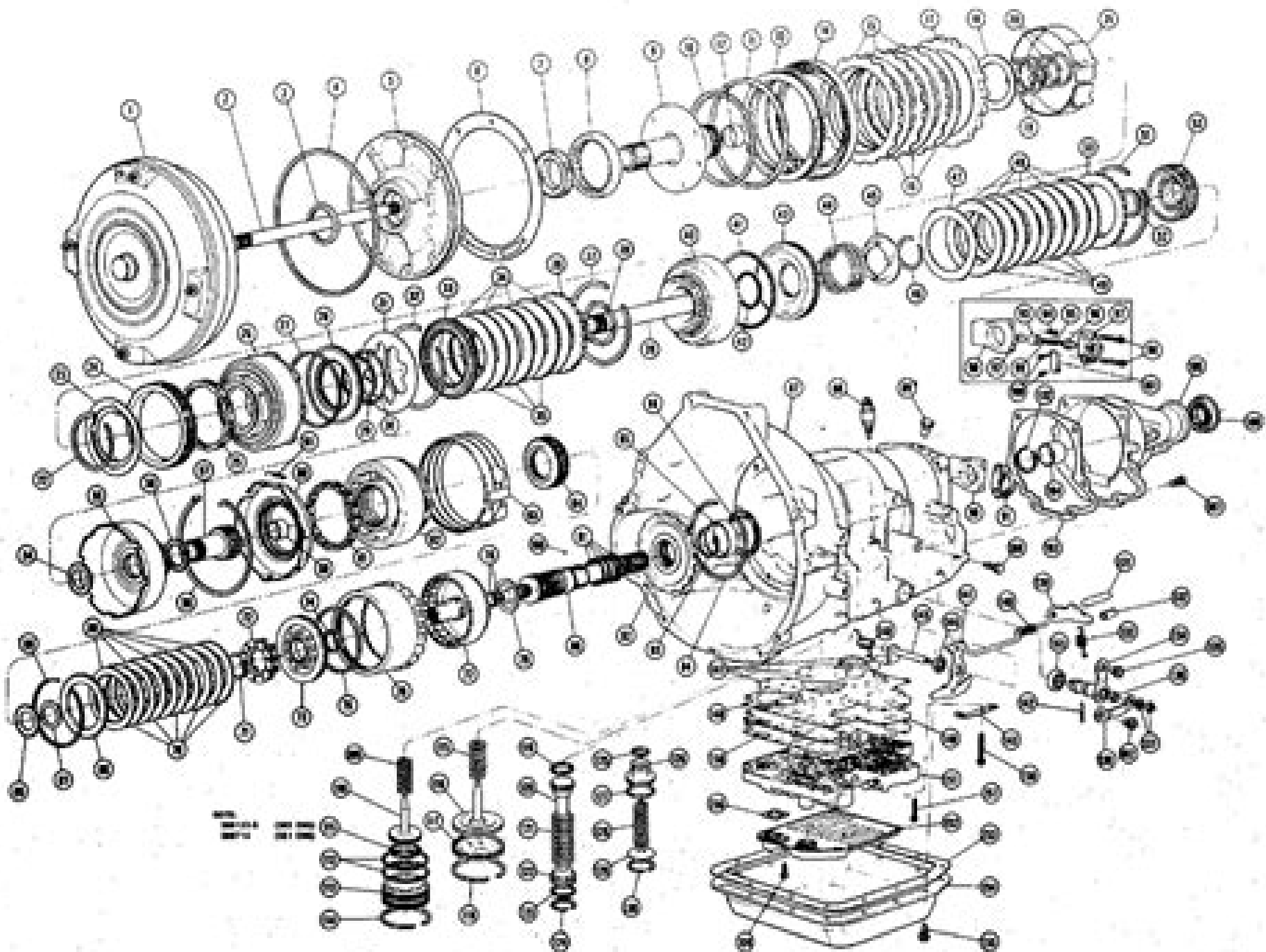
The Ranger Station - Exploded View Of AGO Transmission
