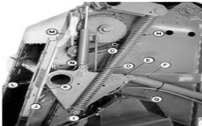
Attach Hoist to Tension Arm Center Roll
