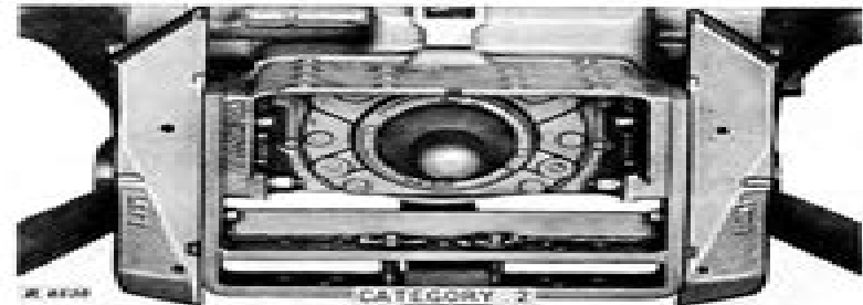
Sway Blocks Installed to Eliminate Side Sway
