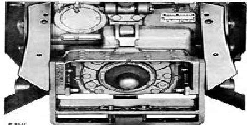
Sway Blocks in Upper Position to Permit Side Sway When Implement Is Working (Category 2 Implement)
