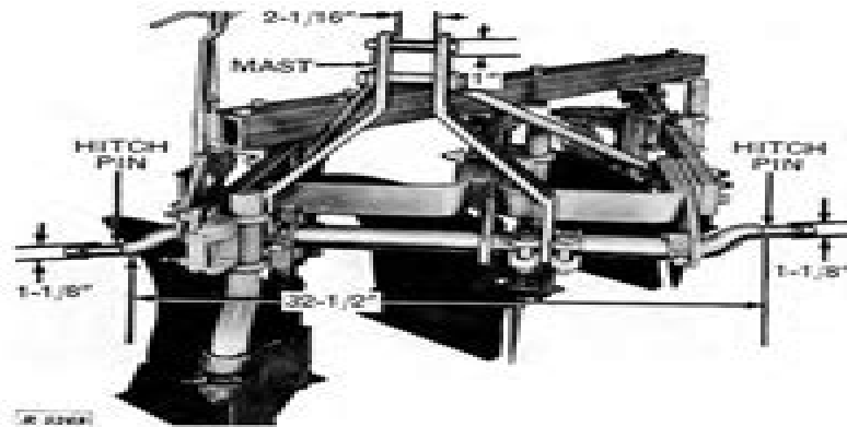
Category 2 Implement Hitch Dimensions
