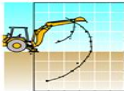
210SE BACKHOEWITH 3-FT. 6-IN. (1.07 M) EXTENDABLE DIPPERSTICK, RETRACTED
