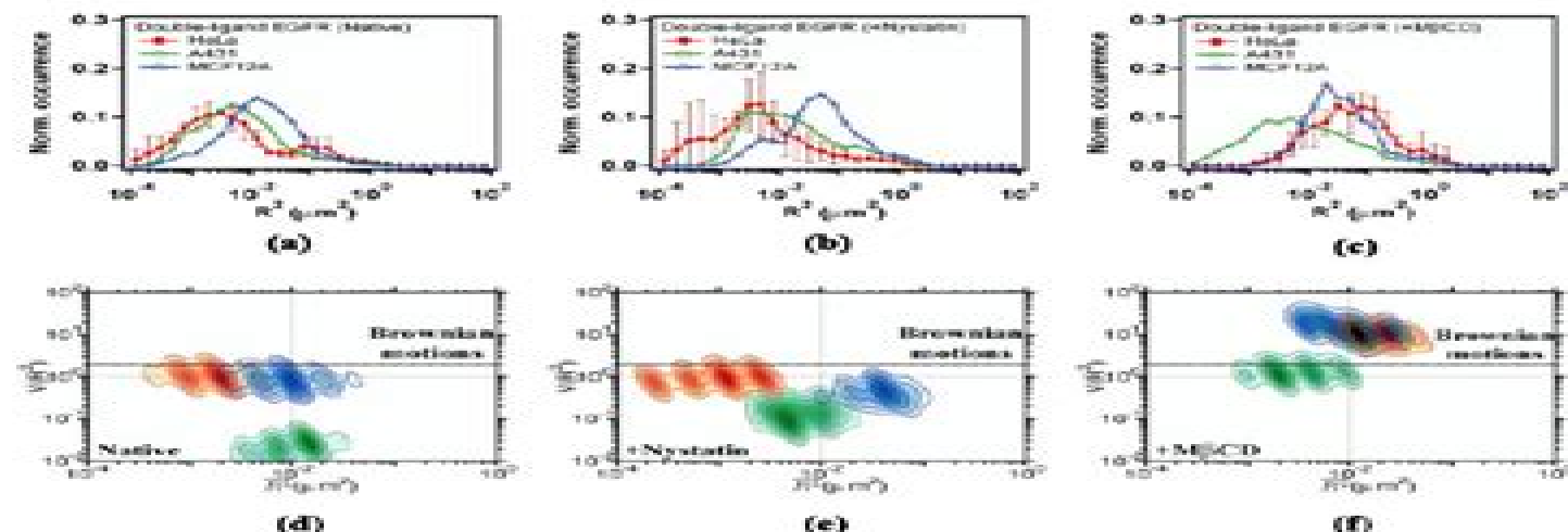
Fig. 6 a, b, c Histograms of MSDs and (d, e, f) V(\overline{R_r^{-2}}) - \overline{R_r^{-2}} plots of correlated Qdot585-EGF-EGFRs diffusing in the plasma membrane of (a, d) native cells, (b, e) nystatin-pretreated cells, and (c, f) M \beta CD-pretreated cells. Trajectory segments with a degree of correlation exceeding 0.8 were analyzed. Trajectories were sampled with a frame period of \tau=25 ms. Data are shown in red for HeLa cells, green for A431 cells, and blue for MCF12A cells.
