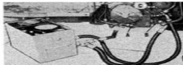
Fig. 5—View showing Flow-Relief connected for testing hydraulic flow and pressure.
