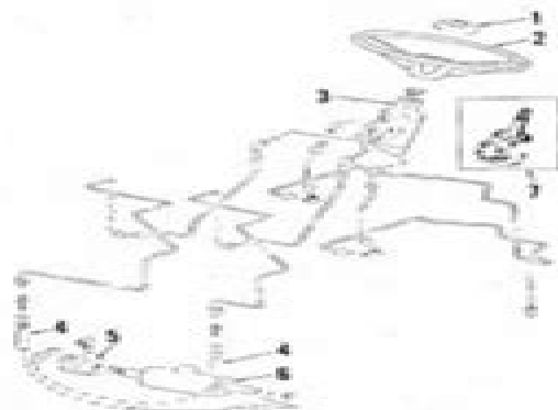
Fig. 3—Schematic view showing general layout of component parts of typical power steering system on International tractors. Hand pump and steering valve (3) is used on Models 434, 484, 574 and 574. Dashco pump and steering valve (7) is used on Models 484 and 584.
