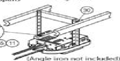
Figure 6 Mounting methods for open beam and finished ceilings
