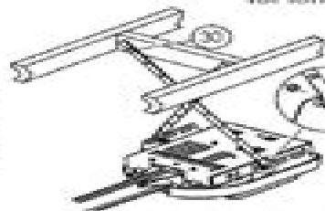
Figure 6 Mounting methods for open beam and finished ceilings
