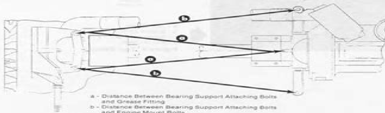
Figure 2. Engine Alignment
