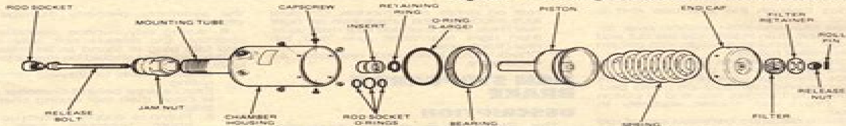
Fig. 40 Exploded view of parking brake chambers. Ford
