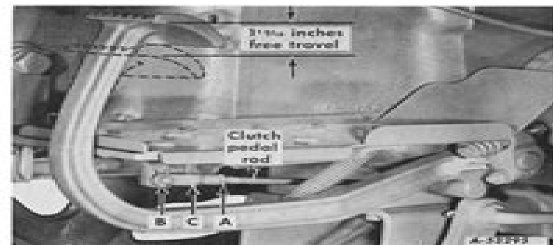
Illustr. 39A Clutch pedal free movement.
