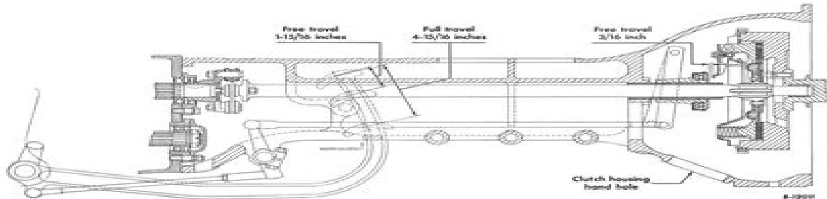
Illustr. 39 Clutch and connections.
