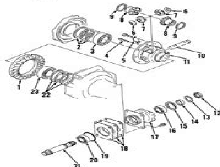
Fig. 8—Exploded view of four-wheel drive front differential used on Model 234.
