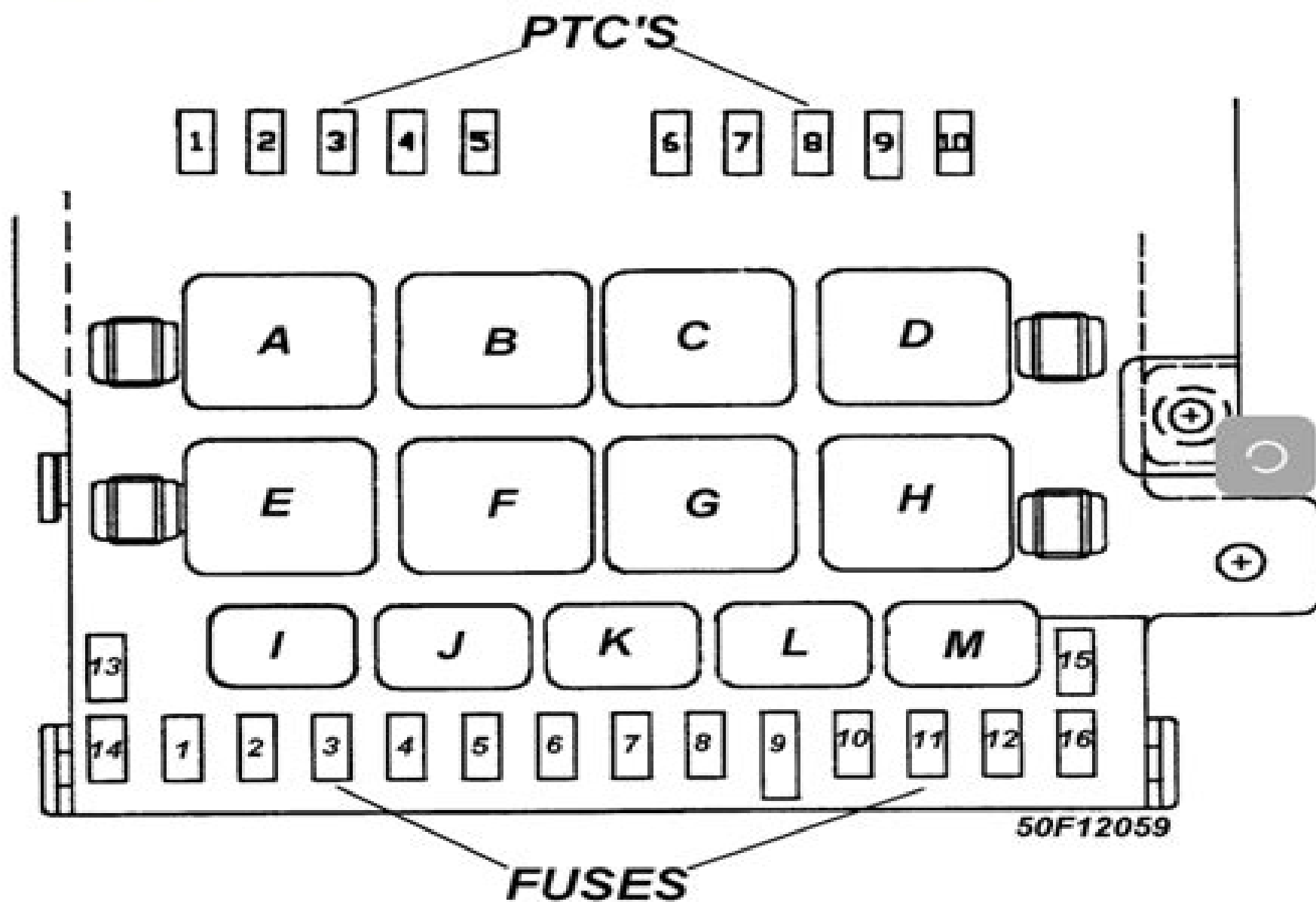
Fig 1: Fuse Panel Identification
