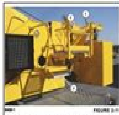
Use the hoist access platform (1) (Figure 2-11) when working in the hoist area (2) (hoist counterweight units only).
