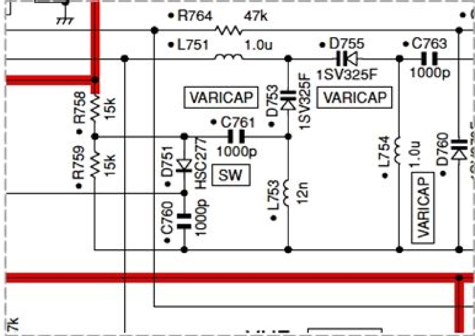
Preview: KENWOOD TM-D710A schematic diagram
