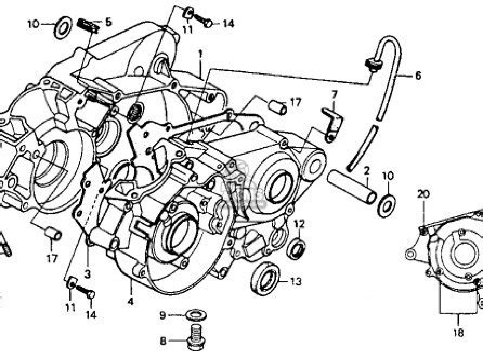
CRANKCASE
