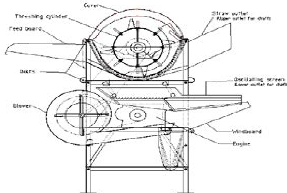
Fig. 3. Thresher JEP
