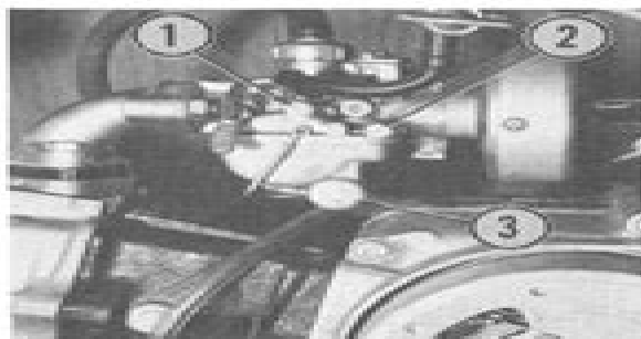
Fig. 2—Carburetor may be drained by turning drain plug (3). For adjustment of speed screw (1) and idle mixture needle (2), refer to engine section.
