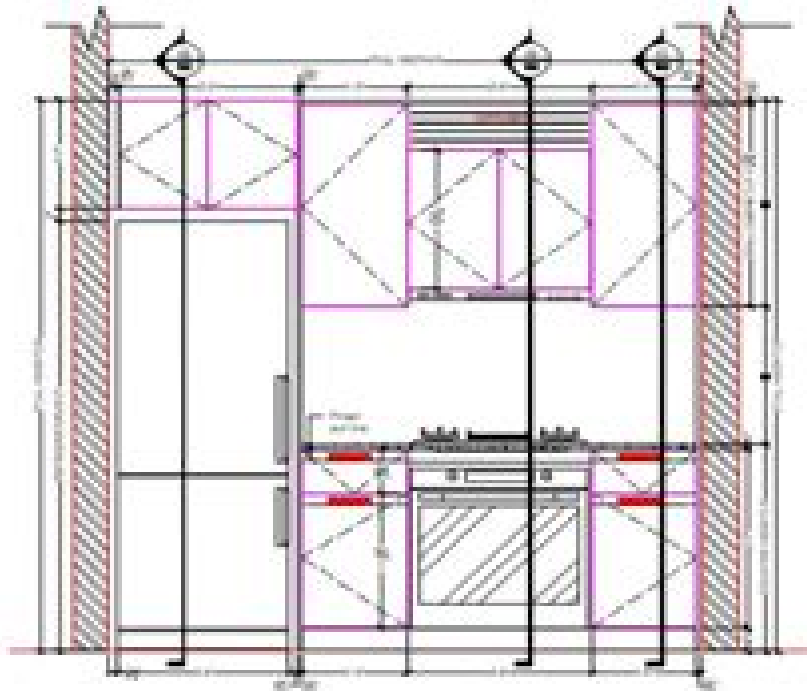
04 ELEVATION-01 FRONT ELEVATION (U.A.E)
