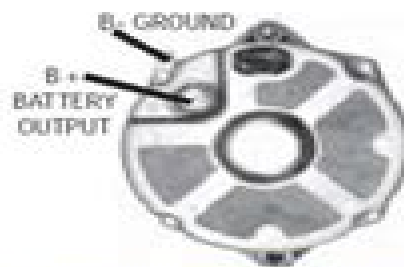
DELCO SELF EXCITING STYLE FITS MERCURUISER AND OMC
