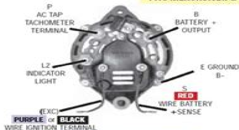
LATE MANDO STYLE FITS MERCURUISER AND OTHERS
