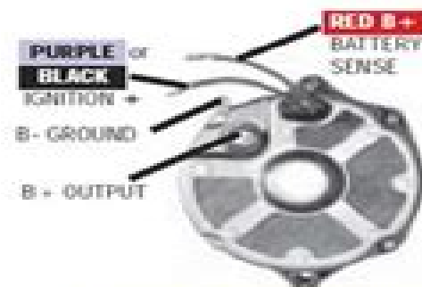
DELCO STYLE FITS MERCURUISER & OMC
