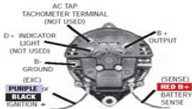
LATE MOTOROLA/PRESTOLITE STYLE FITS MERCURUISER & OMC
