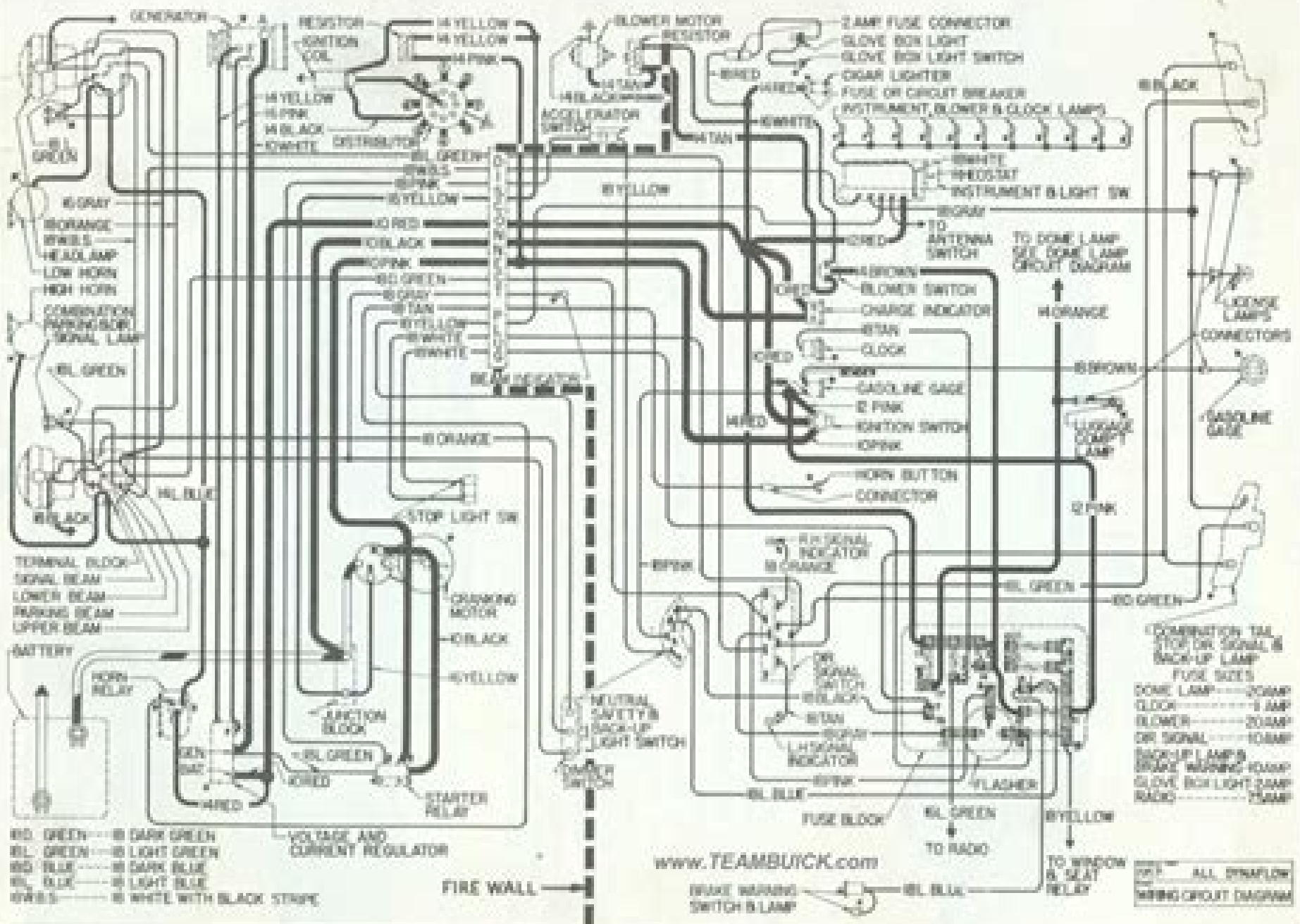
Figure 10-77—Chassis Wiring Diagram (Continued)
