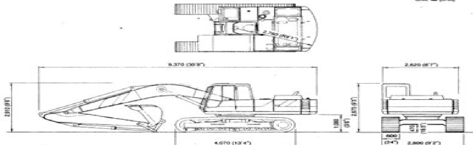
K907 - II 2.94 m (9 ft-7 in) ARM (STD)
