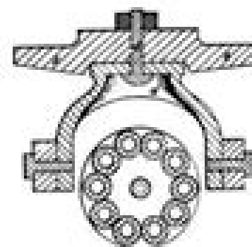
FIG. 5. SECTION THROUGH GUN WITH CARTRIDGE CHAMBER AND PIVOT BLOCK.
