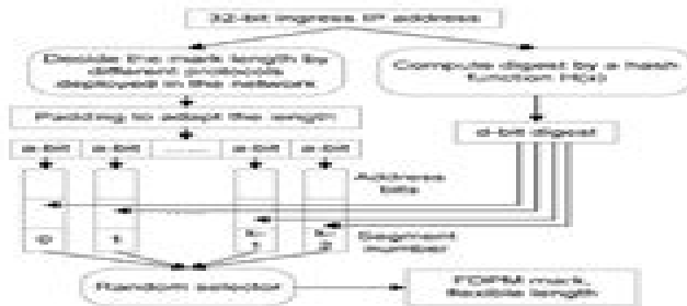
Fig. 3: FDPM encoding procedure
