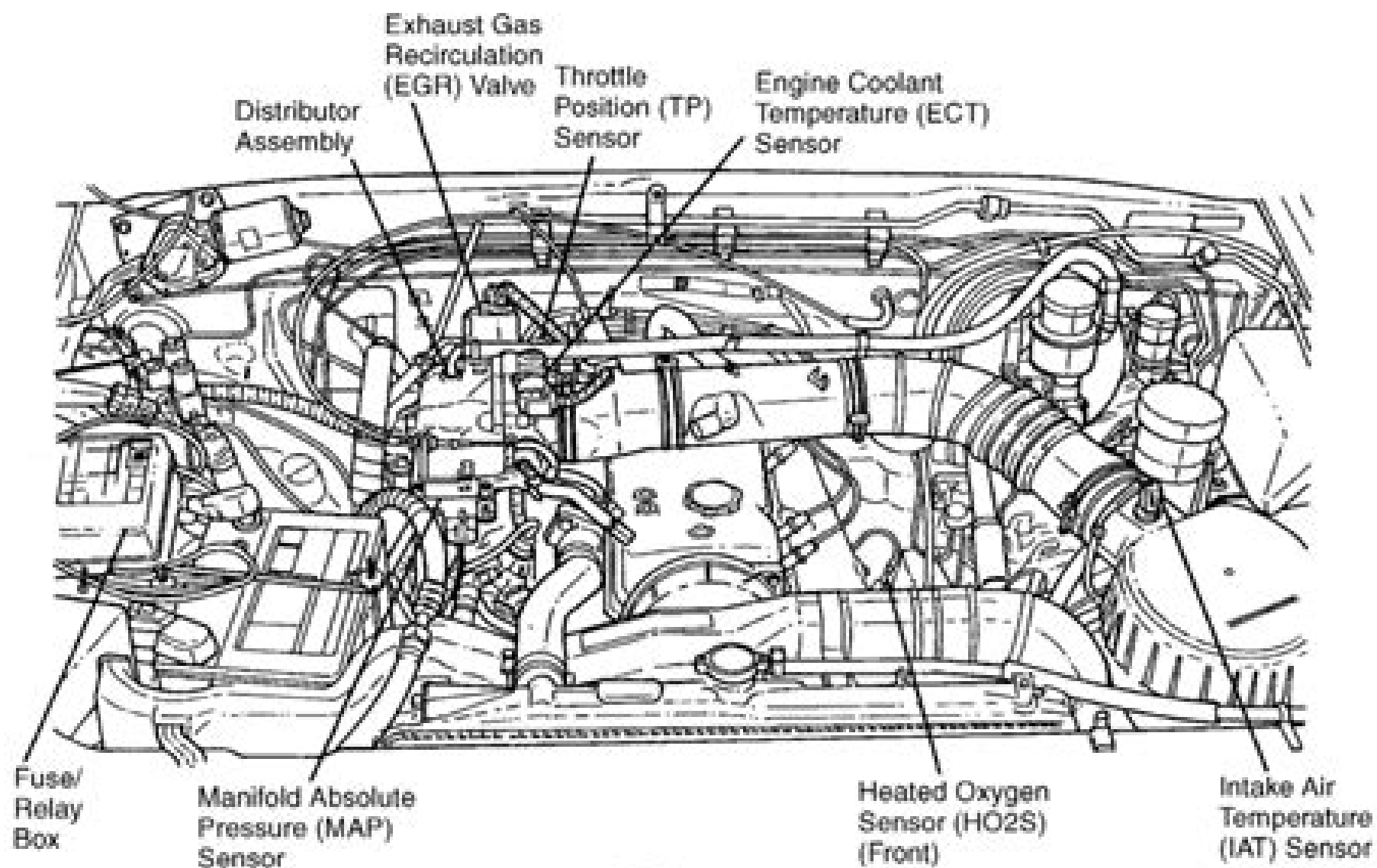
Fig. 1: Engine Compartment (2.6L)
