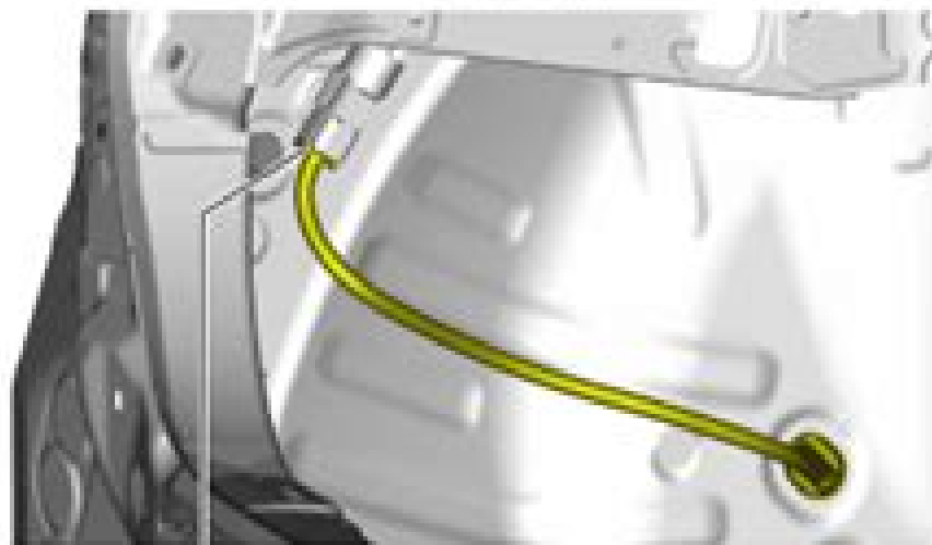
REAR ABS WHEEL-SPEED SENSOR CONNECTOR
