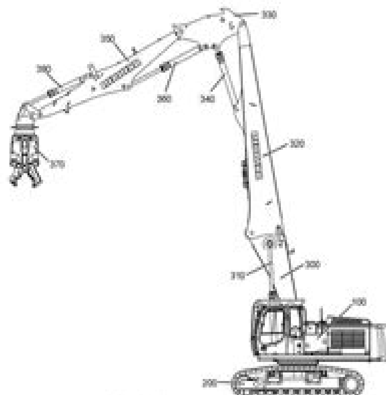
Fig. 1-2 Machine with demolition attachment
