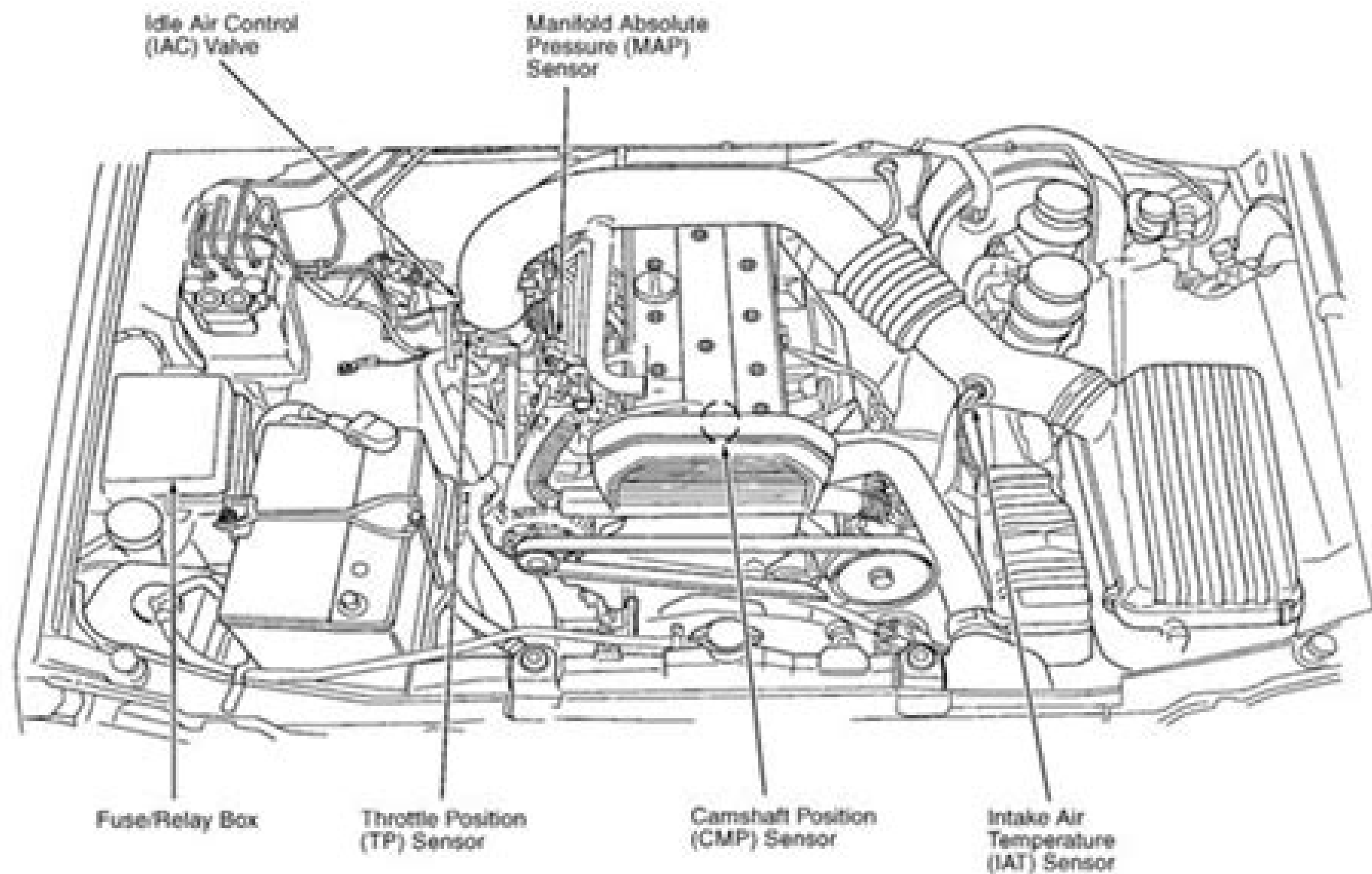
Fig. 1. Engine Compartment (2.2L)
