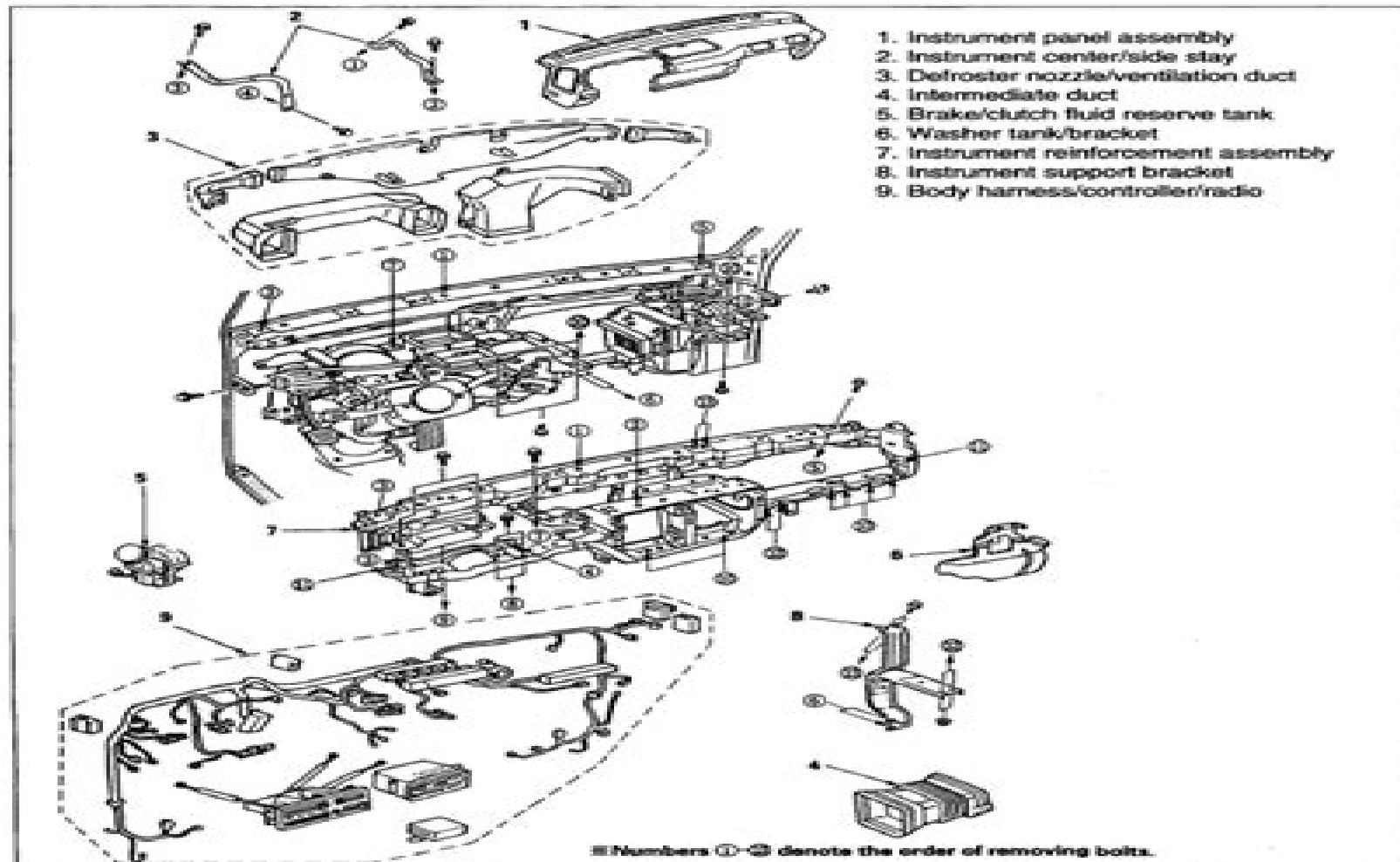
Figure 21. Instrument Panel Reinforcement Removal or Installation
